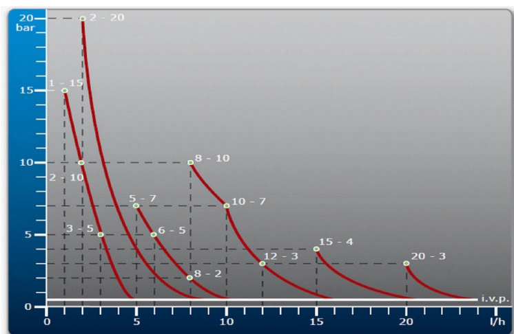
Pressure (bar) – Flow Rate (l/h) Chart
